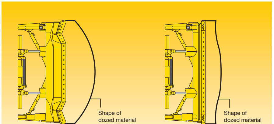
Up to 15% higher productivity with the improved Sigmodozer® blade (left), compared to conventional Semi-U blade (right)
